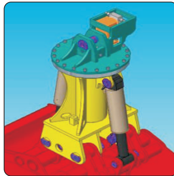
Heavy duty over size pins & spring steel bushes give better life of bucket.
