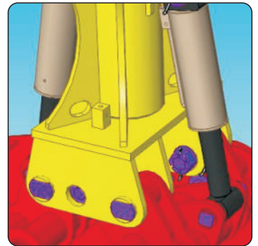
Heavy duty hydraulic cylinders with extra wall thickness body.
